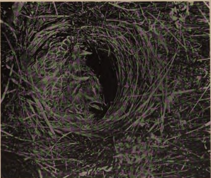
FIG. 46. Young Western Meadowlark in their ground nest. 'Grass-pattern' birds. Photographed from life by Pinoy & Hobman.
